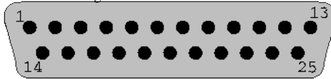
Figure 2 – RS-232 Connector
