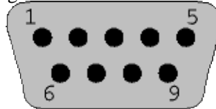
Figure 4 – RS-574 Connector
